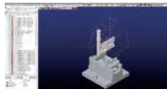
HyperMILL CAD/CAM
